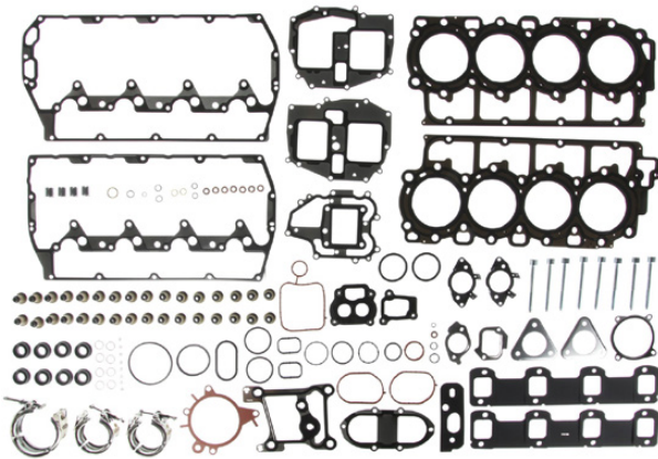
Ford 6.7L Cylinder Head Gasket Set
